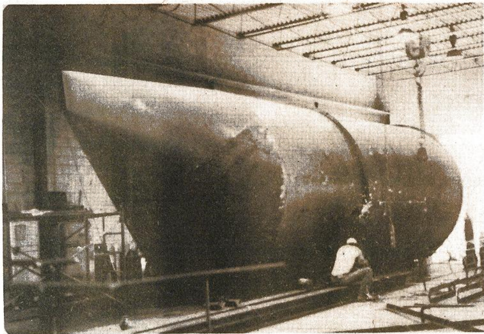
Custom bulk storage tank in process of fabrication for Malartic Gold Mines.
